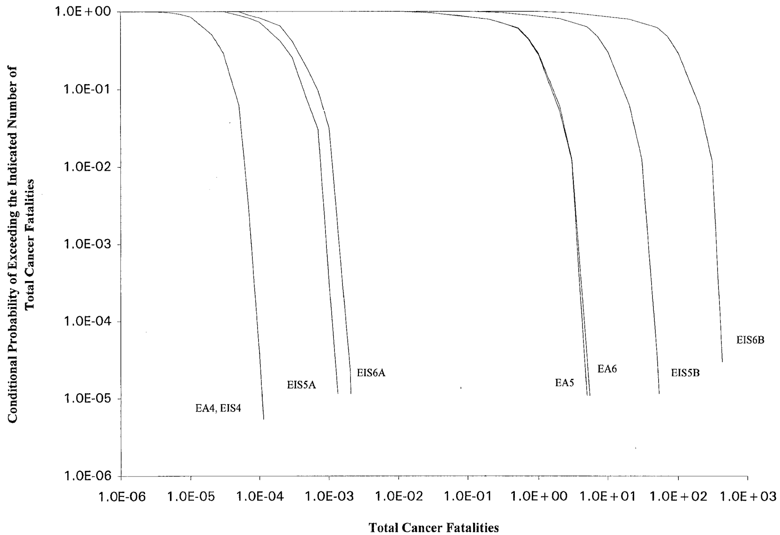
Figure 65. Total Cancer Fatalities, 0-80 km, Tacoma Dock, BR-2 Inventory, All EA and EIS Source Terms, Variable Meteorology
