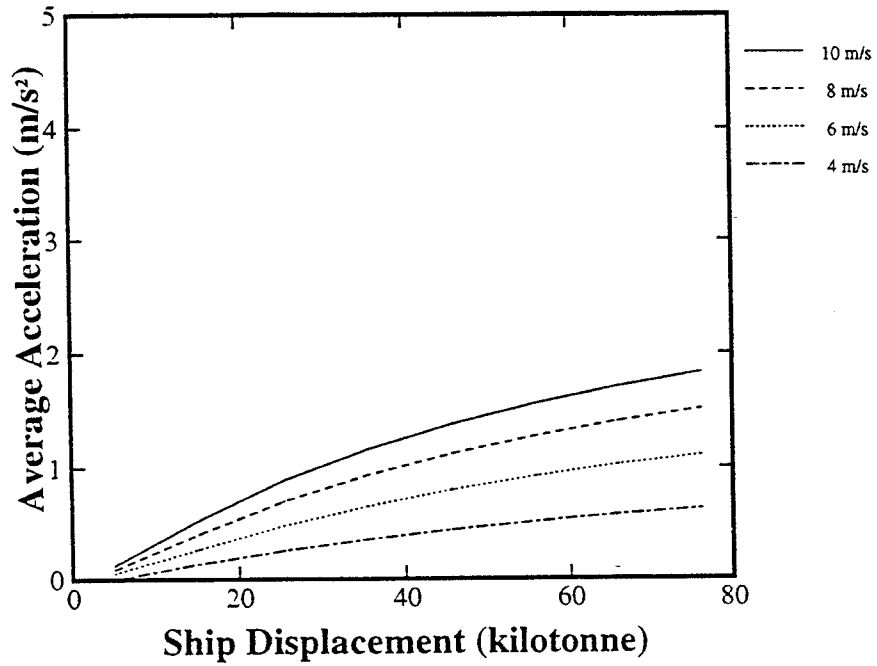
Figure 12. Average Accelerations for the Medium Cargo Case ( f = 0.2 , \sigma = 34.5 MPa)
